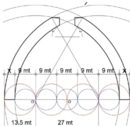
Figure 6: Pointed arches [4]
