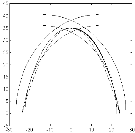
Figure 7: Catenary through (0,35), (24,0)
