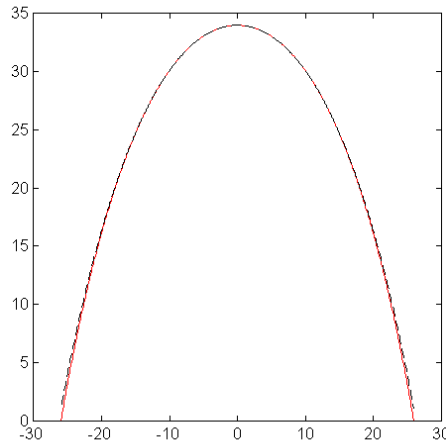
Figure 2: Catenary and approximating parabola
