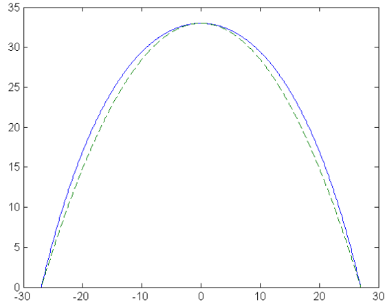
Figure 3: Catenary and interpolating parabola
