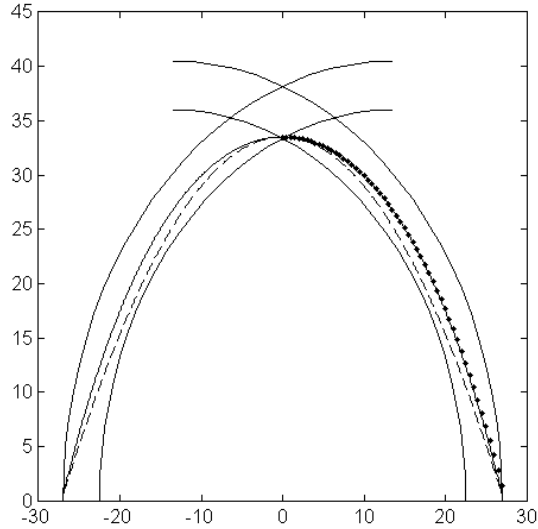
Figure 8: Catenary through (0,33.5) , (27,0)
