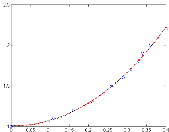
Figure 5: Fitting experimental data by catenary and parabola
