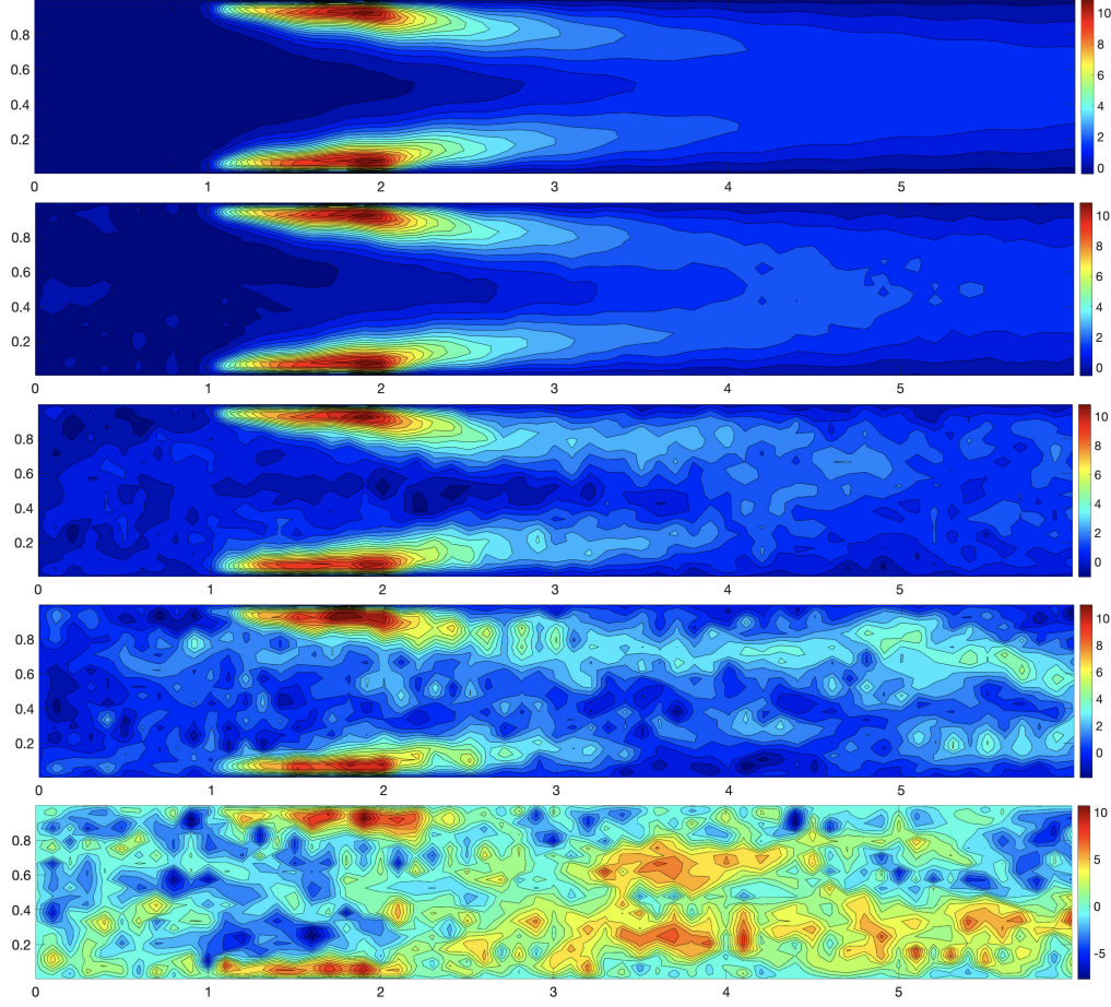
Figure 3: Test case 2. HiMod reference solution (top panel); interpolation-HiPOD approximation for different noise levels: \eta = 0.01, 0.05, 0.1, 0.25 (second-fifth row).
