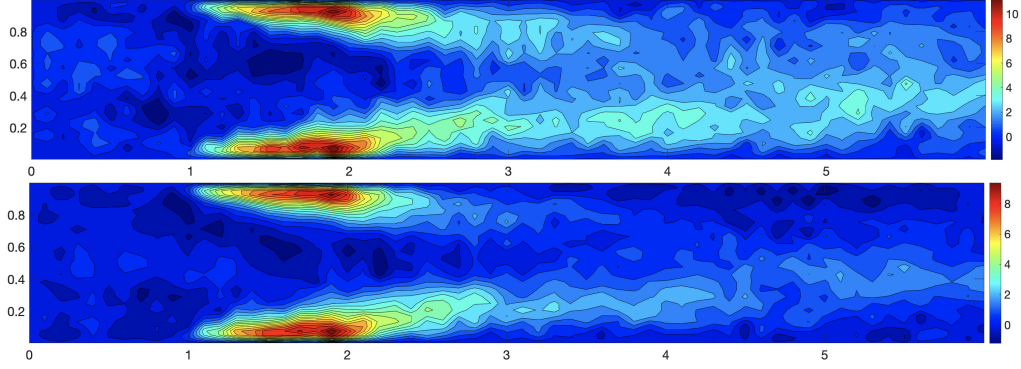
Figure 4: Test case 2. Regression-HiPOD approximation for a cubic polynomial fitting (top) and for a Gaussian process regression (bottom); the noise level is set to \eta = 0.25 .
