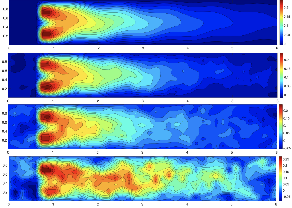
Figure 1: Test case 1. HiMod reference solution (top panel); interpolation-HiPOD approximation for different noise levels: \eta = 0.01, 0.1, 0.25 (second-fourth row).
