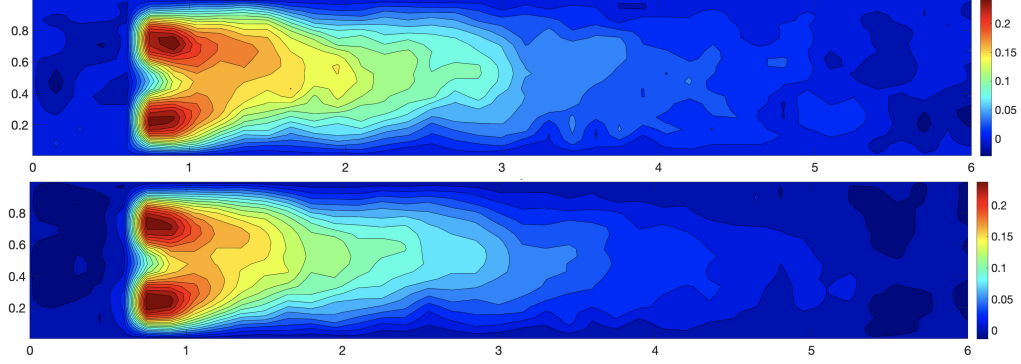
Figure 2: Test case 1. Regression-HiPOD approximation for a cubic polynomial fitting (top) and for a Gaussian process regression (bottom); the noise level is set to \eta = 0.25 .
