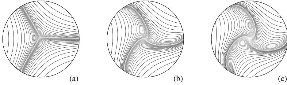
Figure 1: numerical simulations of functions belonging to the class \mathcal{S} for different values of \alpha . In this particular case, we have considered a system of 3 components (labeled in counterclockwise order as u_1, u_2 and u_3 ) in the unit ball, with boundary conditions given by suitable restrictions of |\cos(3/2 \vartheta)| . In picture (a), a_{ij} = 1 for all i, j , which yields \alpha = 0 (see Remark 1.6). In picture (b), a_{ij} = 4 if j - i = 1 \pmod 3 and a_{ij} = 1 otherwise, which yields \alpha = 3 \log 4/2\pi (> 0 , which implies by equation (5) that the free-boundary is described asymptotically by rotations of the clockwise logarithmic spiral \vartheta = \log 4/\pi \log r ). In picture (c), a_{ij} = 10 if j - i = 1 \pmod 3 and a_{ij} = 1 otherwise, which yields \alpha = 3 \log 10/2\pi .
