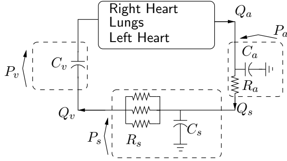
Figure 17: (From [36]). A four compartment description of the vascular system with self-regulating controls.
