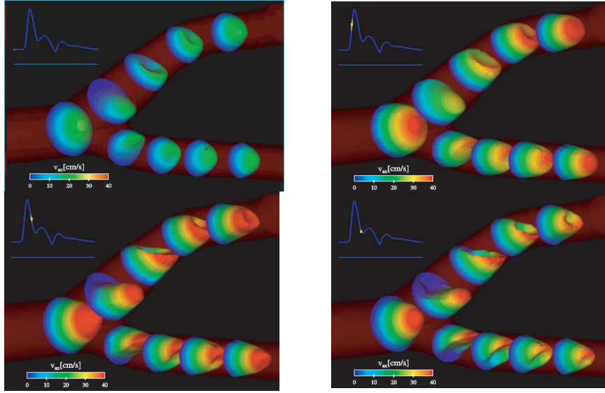
Figure 6: Velocity profiles computed in a carotid bifurcation during systole and diastole (courtesy of M. Prosi).
