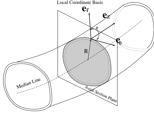
Figure 8: A model of a “realistic” section of an artery with the principal geometrical parameters.
