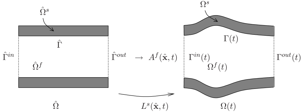
Figure 9: Parametrization of the domain.
