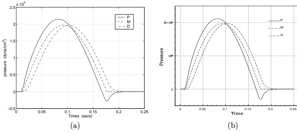
Figure 5. Time history: (a) Taylor-Galerkin and (b) discontinuous Galerkin schemes.
