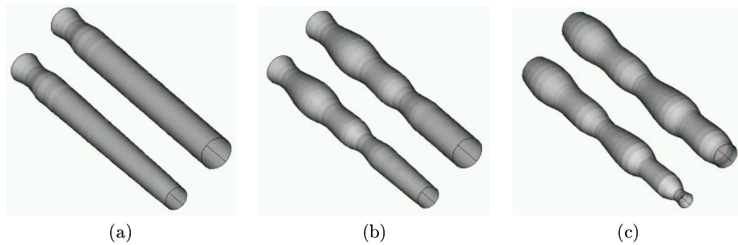
Figure 10. Three dimensional interpretation of waves in normal (top) and tapered (bottom) vessels (a) t = 2.5 , (b) t = 12.5 and (c) t = 20 . The displacement from A_0(x) has been magnified by a factor of 10 and the x -axis is scaled by a factor of 1/20 .
