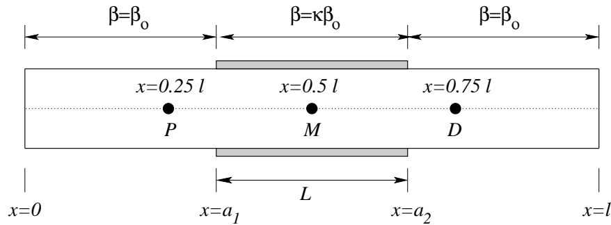
Figure 3. Test case layout.
