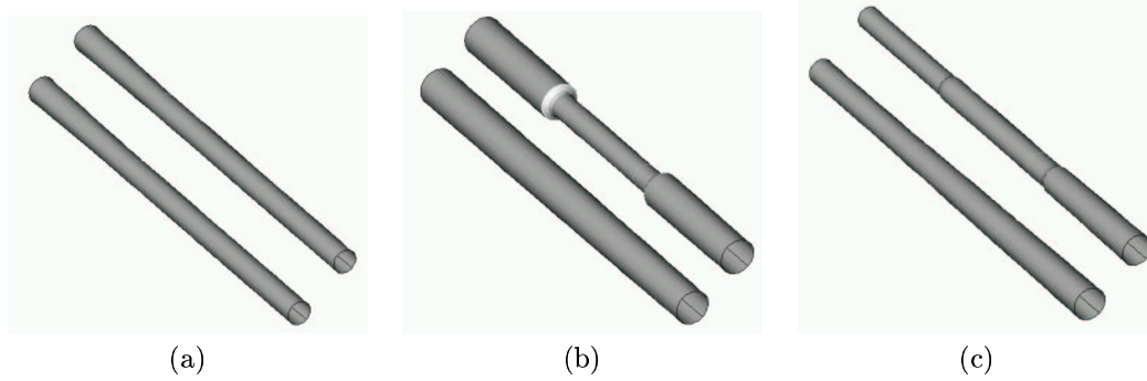
Figure 6. Three dimensional interpretation of waves in stented (top) and normal vessel (bottom) (a) t = 0.01 , (b) t = 0.075 and (c) t = 0.175 . The displacement from A_0 has been magnified by a factor of 10.
