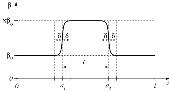
Figure 4. Variation of wall properties in test case.
