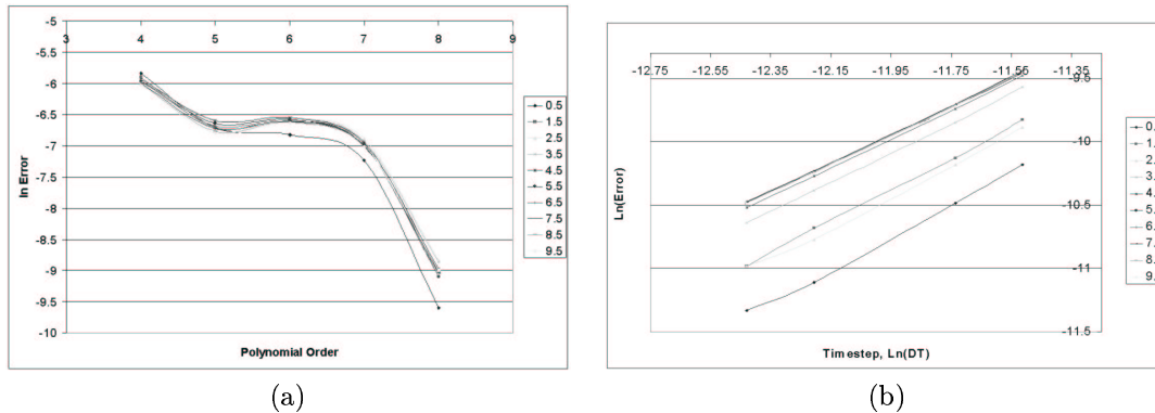
Figure 15. Logarithmic plot of velocity error at a point in the abdominal aorta (artery 39) against: (a) polynomial order and (b) timestep.
