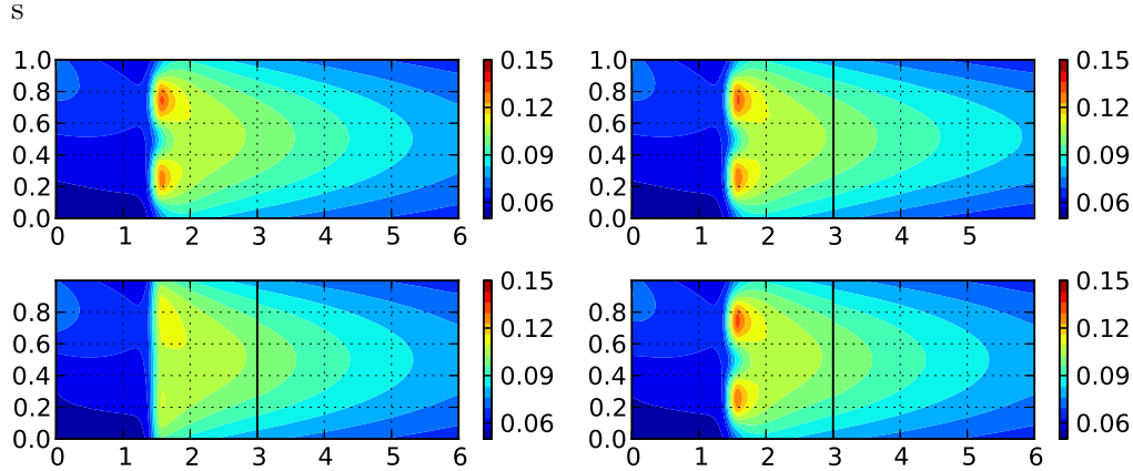
Figure 3: Full solution (top-left); geometrical multiscale solution (top-right) and Hi-Mod solution with \{3, 1\} (bottom-left) and \{5, 1\} (right) modes
