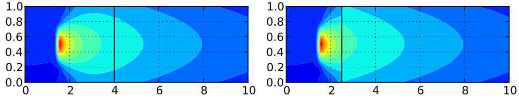
Figure 2: Piecewise Hi-Mod reduction: reduced solutions associated with \{5, 2\} modes, the interface is \Gamma_4 (on the left) and \Gamma_{2.5} (on the right); h = 0.05 on \Omega_{1D}
