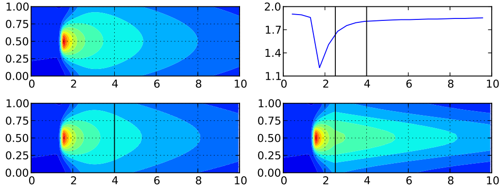
Figure 1: Geometrical multiscale: full solution (top-left); graph of \sigma_r (top-right); coupled solution for \Gamma_4 (bottom-left) and \Gamma_{2.5} (bottom-right)
