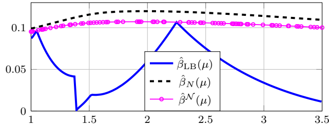
Figure 3: Test 1: lower bound for the Babuška inf-sup constant \hat{\beta}^{\mathcal{N}}(\boldsymbol{\mu}) as a function of the geometrical parameter \mu_1 (on the x-axis).
