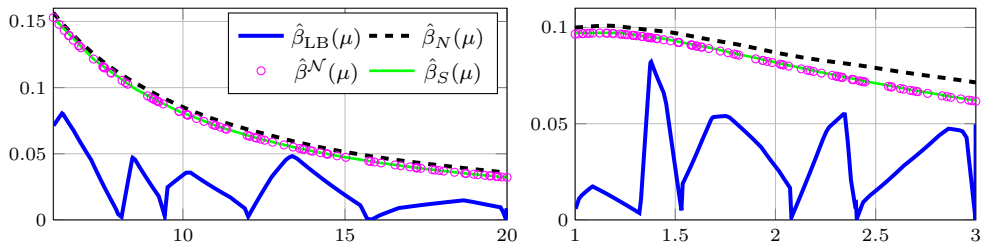
Figure 11: Test 3: comparison between lower bound and interpolant surrogate for the discrete Babuška inf-sup constant \hat{\beta}^{\mathcal{N}}(\boldsymbol{\mu}) . On the left: \hat{\beta}^{\mathcal{N}}(\boldsymbol{\mu}) as a function of \mu_1 , (\mu_2, \mu_3) = (1.5, 3) fixed; on the right: \hat{\beta}^{\mathcal{N}}(\boldsymbol{\mu}) as a function of \mu_2 , (\mu_1, \mu_3) = (9, 1) fixed.
