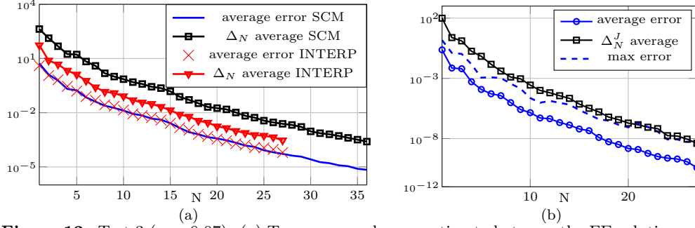
Figure 12: Test 3 ( \alpha = 0.07 ). (a) True error and error estimate between the FE solution and the RB approximation: the quantities in red are obtained using the interpolant surrogate \hat{\beta}_S(\boldsymbol{\mu}) instead of \hat{\beta}_{LB}(\boldsymbol{\mu}) . (b) Average true error and bound \Delta_N^J(\boldsymbol{\mu}) between \mathcal{J}^N(\boldsymbol{\mu}) and \mathcal{J}_N(\boldsymbol{\mu}) using \hat{\beta}_S(\boldsymbol{\mu}) in the estimate.
