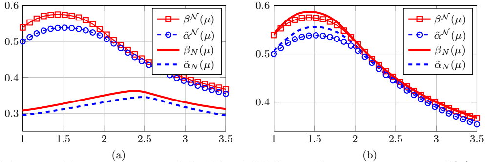
Figure 4: Test 1: comparison of the FE and RB discrete Brezzi inf-sup constant \beta(\boldsymbol{\mu}) and coercivity constant of the state equation \tilde{\alpha}(\boldsymbol{\mu}) . The two quantities are given as function only of \mu_1 , since \mu_2 does not appear in the affine expansion of \mathcal{B}(\cdot, \cdot; \boldsymbol{\mu}) . (a) No enrichment: Y_N \neq Q_N . (b) Aggregated space: Y_N = Q_N = Z_N with Z_N defined as in (20).
