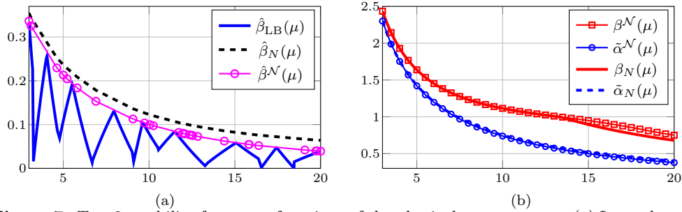
Figure 7: Test 2: stability factors as functions of the physical parameter \mu_1 . (a) Lower bound for the discrete Babuška inf-sup constant \hat{\beta}^N(\mu) . (b) Comparison of discrete Brezzi inf-sup constant \beta(\mu) and coercivity constant \tilde{\alpha}(\mu) for the FE and RB approximations.
