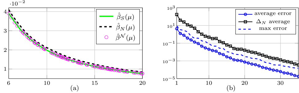
Figure 13: Test 3 ( \alpha = 8 \cdot 10^{-3} ). (a) Interpolant surrogate for the discrete Babuška inf-sup constant \hat{\beta}^N(\boldsymbol{\mu}) as a function of \mu_1, (\mu_2, \mu_3) = (1.5, 3) fixed. (b) Average and max true errors and estimate on the solution variables.
