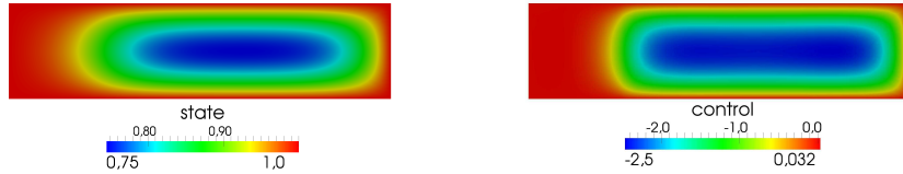
Figure 2: Test 1: representative solution for \boldsymbol{\mu} = (0.6, 3) ; on the left the state variable y_N , on the right the optimal control u_N .
