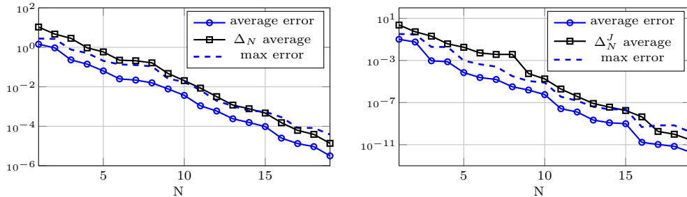
Figure 8: Test 2. Average and max computed errors and bound between the truth FE solution and the RB approximation (left). Average true error and bound \Delta_N^J(\mu) between \mathcal{J}^N(\mu) and \mathcal{J}_N(\mu) (right).
