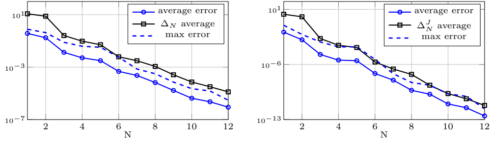
Figure 5: Test 1. Average and max computed errors and estimate between the truth FE solution and the RB approximation, for N = 1, \dots, N_{max} (left). Average computed errors and estimate \Delta_N^J(\mu) between \mathcal{J}^N(\mu) and \mathcal{J}_N(\mu) , for N = 1, \dots, N_{max} (right). Here \Xi_{train} is a sample of size n_{train} = 1000 and N_{max} = 12 .
