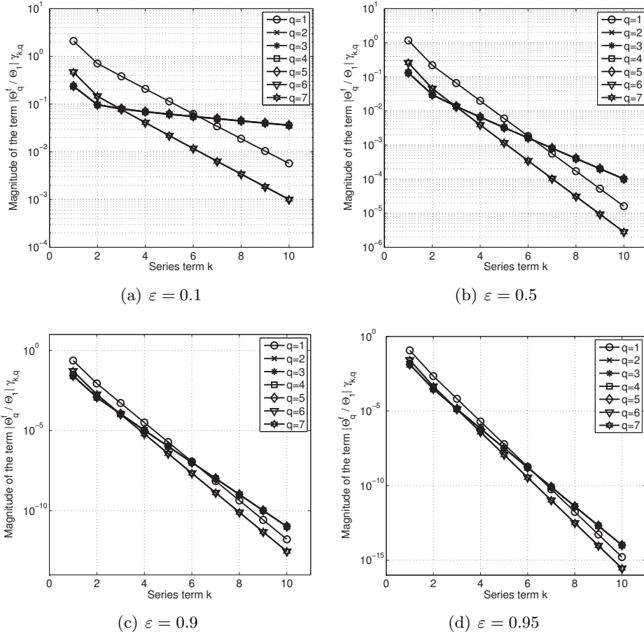
Figure 3: Convergence of the fundamental series (25) coefficients for different values of \varepsilon in (28).
