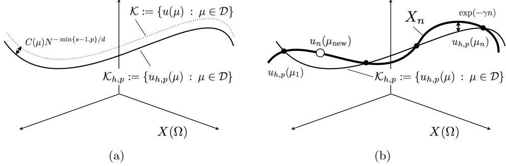
Figure 1: (a) Low-dimensional manifold \mathcal{K}_{h,p} on which the field variable resides and (b) approximation of a new solution at \mu_{\text{new}} with the ‘‘snapshots’’ u_{h,p}(\mu_m) , 1 \leq m \leq n .
