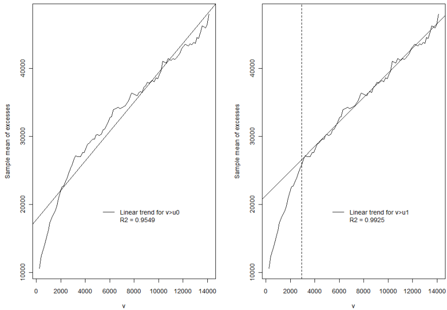
Figure 2: Graph of the empirical means of the excesses with respect to the variation of the threshold above u_0 , considering the linear trends starting the regression respectively from u_0 and from u_1 .
