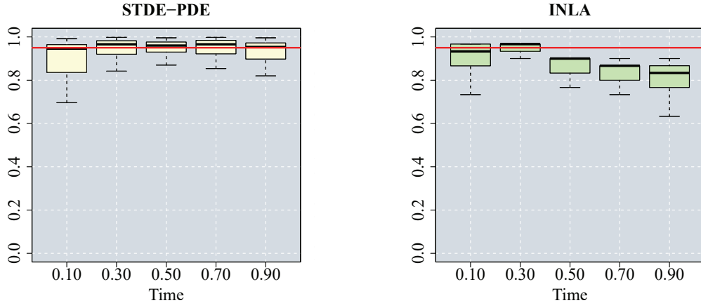
Figure 6: Simulation 1. Boxplots of empirical coverage probabilities of 95% confidence intervals over 30 simulation repetitions: STDE-PDE (left) and INLA (right).
