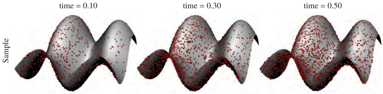
Figure H.1: Simulation 6: point pattern on a non-spherical two-dimensional manifold. Front view of the sample at different time instances over the temporal domain [0, 1] .
