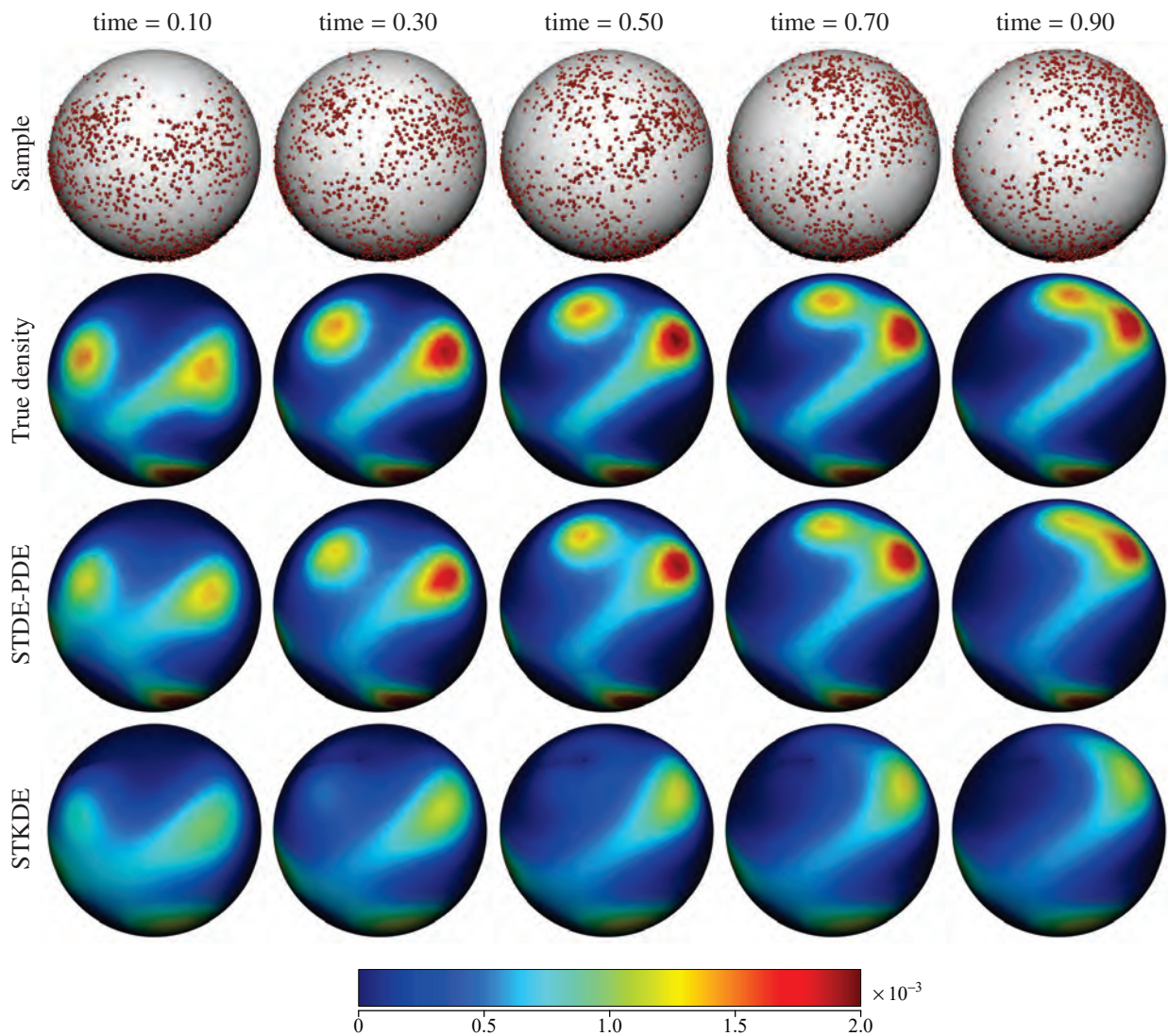
Figure 7: Simulation 2. Front view of the sample (first row), true density (second row), and mean estimates of STDE-PDE (third row), STKDE (fourth row), over 30 simulation repetitions, at different time instances. All the plots have the same color scale, with bluish colors corresponding to low density values.
