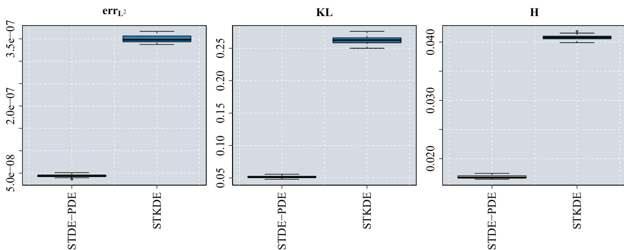
Figure 8: Simulation 2. Boxplots of L^2 -norm of the error (left), Kullback-Leibler divergence (center) and Hellinger distance (right) of the estimates provided by the STDE-PDE and the STKDE methods, over 30 simulation repetitions.
