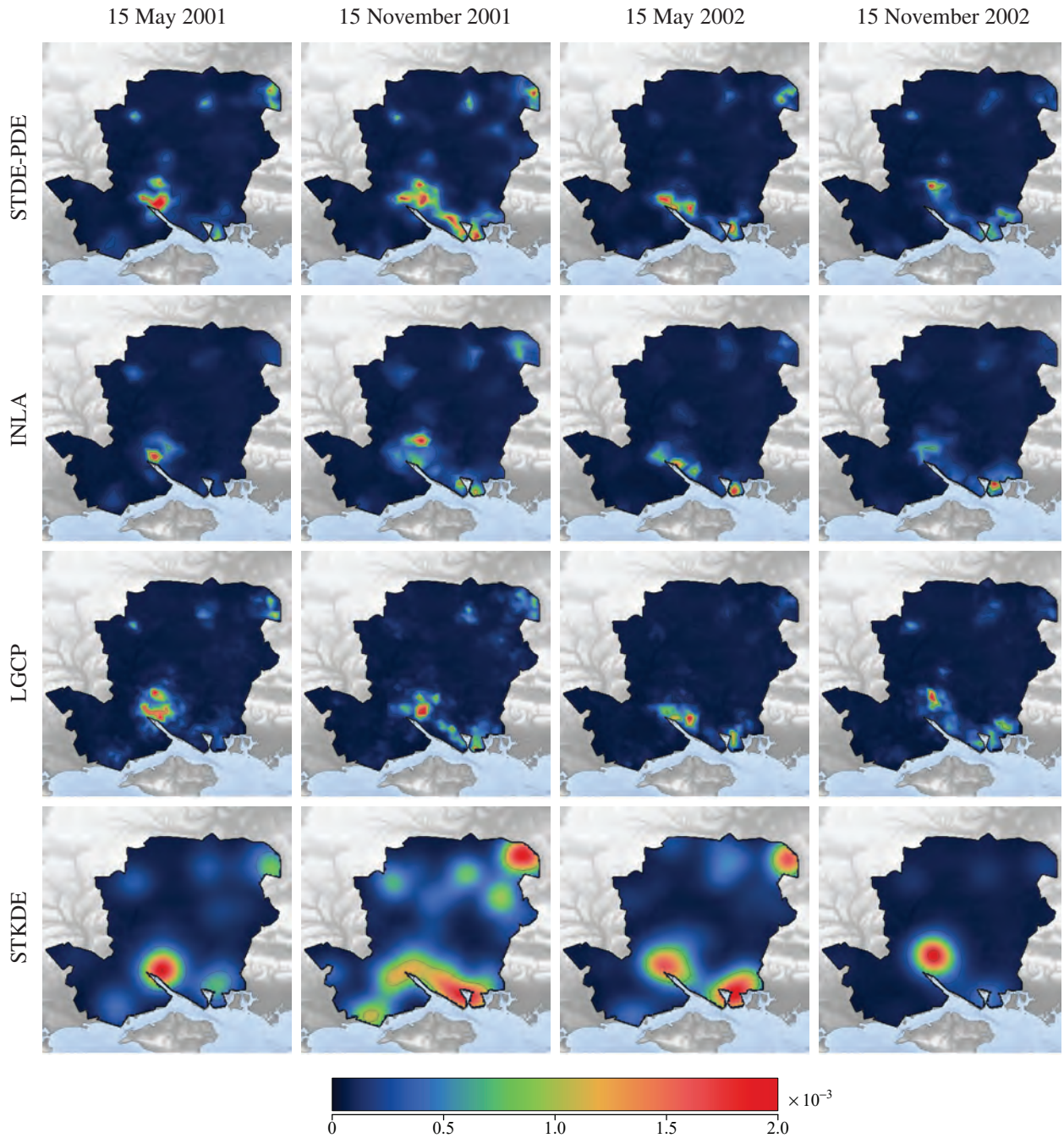
Figure 11: Application to gastrointestinal infections. View of the density estimates for STDE-PDE (first row), INLA (second row), LGCP (third row), and STKDE (fourth row), at different time instances. All the plots have the same color scale, with bluish colors corresponding to low density values of gastrointestinal infections in Hampshire county, UK.
