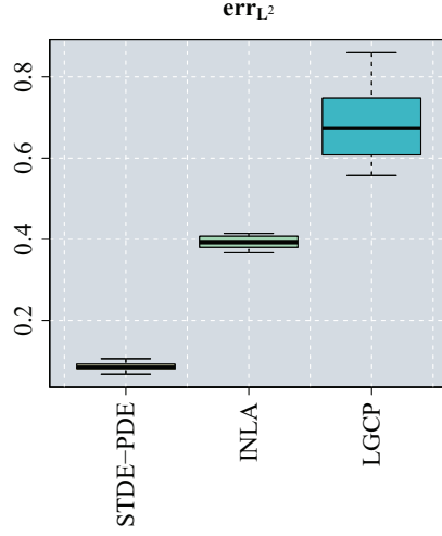
Figure F.1: Simulation 4: intensity estimation of inhomogeneous Poisson Process. Boxplots of L^2 -norm of the error of the estimates of the intensity provided by the proposed STDE-PDE and the considered competing method for intensity estimation, namely INLA and LGCP, over 30 simulation repetitions.
