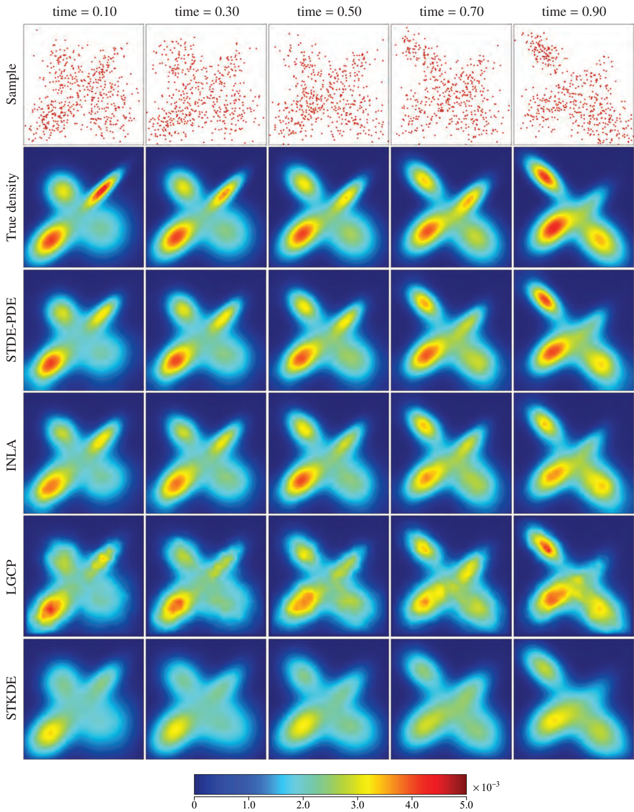
Figure G.2: Simulation 5, additional simulation on planar domain. View of the sample (first row), true density (second row), and mean estimates of STDE-PDE (third row), INLA (fourth row), LGCP (fifth row), and STKDE (sixth row), over 30 simulation repetitions, at different time instances. All the plots have the same color scale, with bluish colors corresponding to low-density values.
