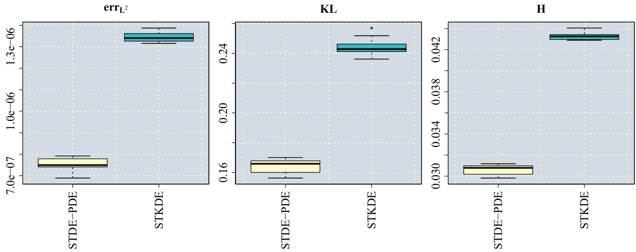
Figure 10: Simulation 3. Boxplots of L^2 -norm of the error (left), Kullback-Leibler divergence (center), and Hellinger distance (right) of the estimates provided by the STDE-PDE and STKDE methods, over 30 simulation repetitions.
