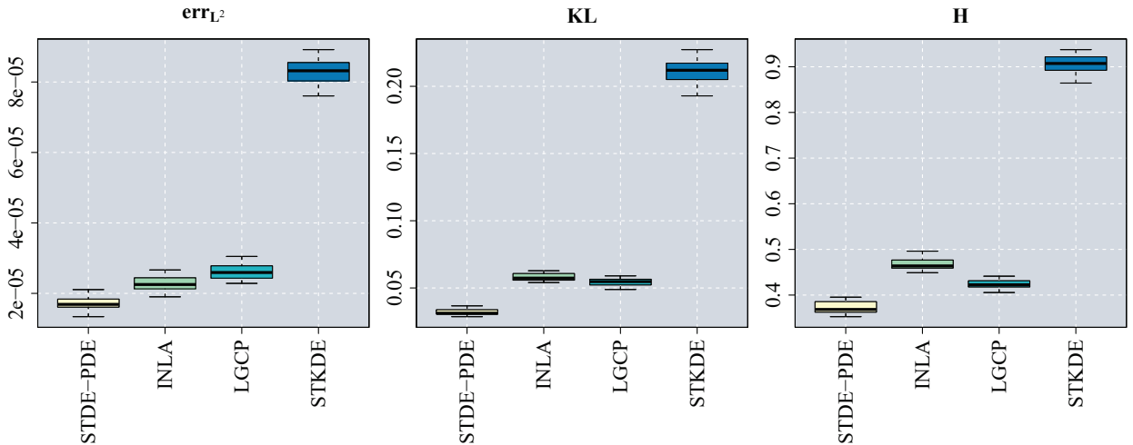
Figure 4: Simulation 1. Boxplots of L^2 -norm of the error (left), Kullback-Leibler divergence (center), and Hellinger distance (right) of the estimates provided by proposed STDE-PDE and the competing methods introduced in Section 6.1, namely INLA, LGCP, and STKDE, over 30 simulation repetitions.
