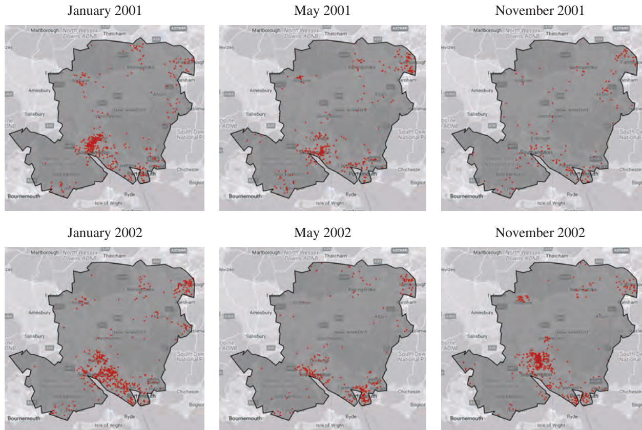
Figure 1: Locations of gastrointestinal infections in Hampshire county, UK, in some months of 2001 and 2002. Although we here plot events on a monthly basis, the data are observed continuously over time (and space). The phenomenon is expressed differently across the irregular spatial domain, resulting for instance in different behaviors along the western and eastern shores of Southampton Water estuary. The background map was obtained using the RgoogleMaps package (Loecher, 2023).
