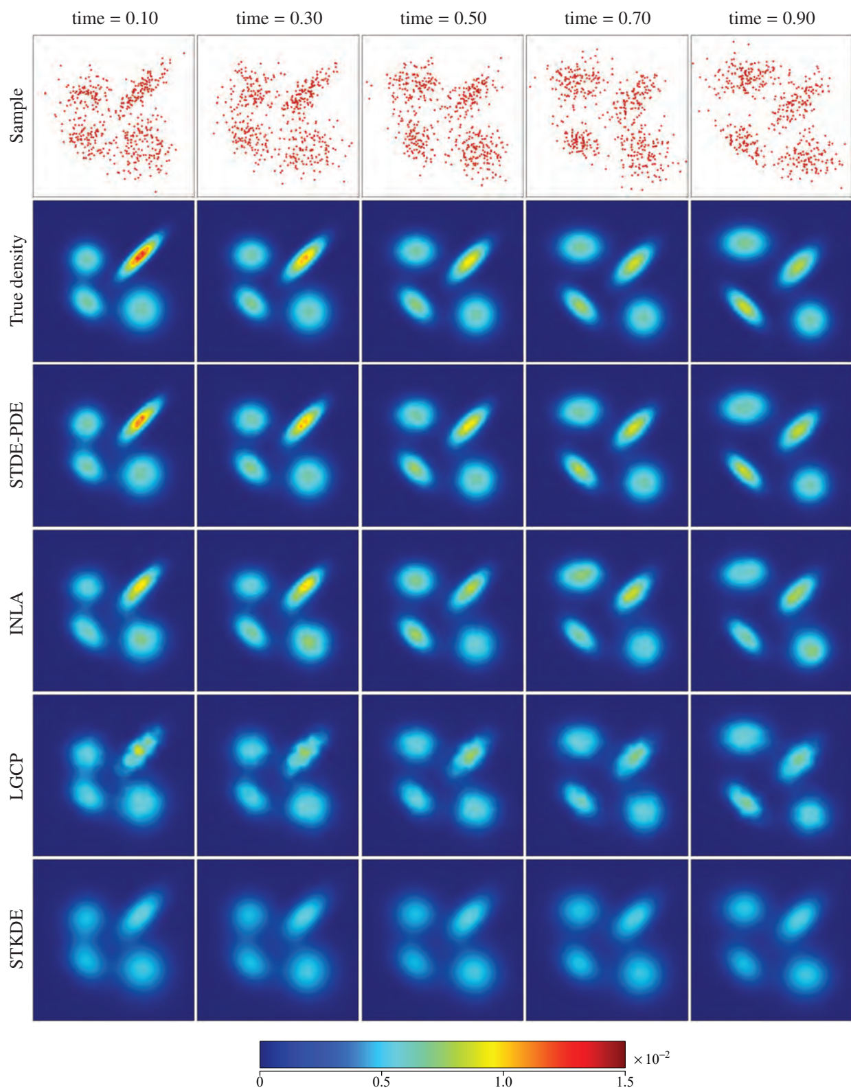
Figure 5: Simulation 1. View of the sample (first row), true density (second row), and mean estimates of STDE-PDE (third row), INLA (fourth row), LGCP (fifth row), and STKDE (sixth row), over 30 simulation repetitions, at different time instances. All the plots have the same color scale, with bluish colors corresponding to low-density values.
