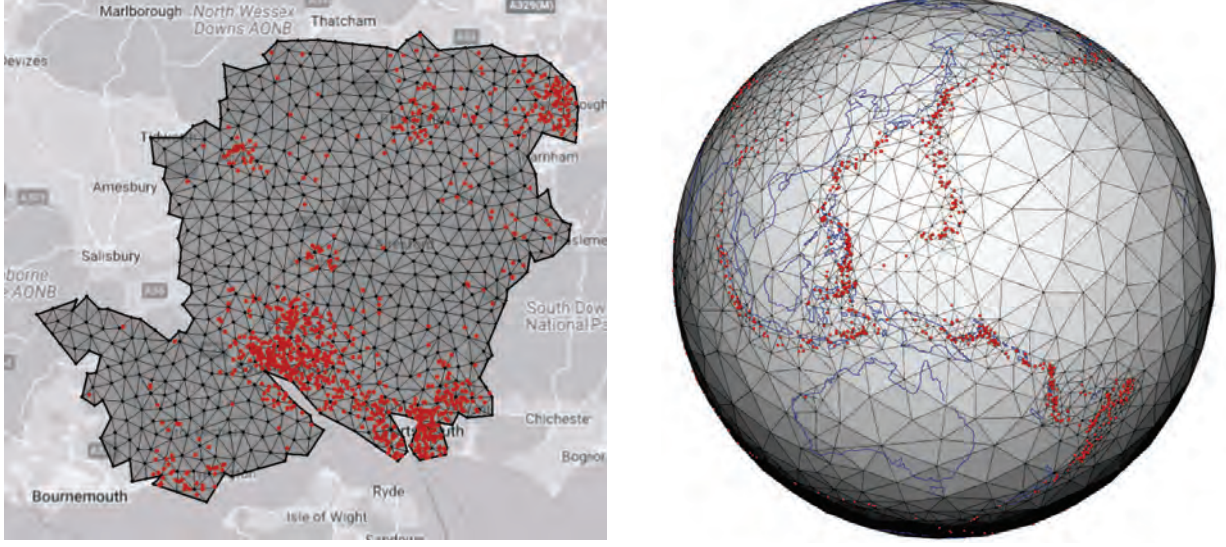
Figure 3: Left: regular spatial mesh with 778 nodes of the Southampton region, Hampshire county, UK. Right: data-driven adaptive spatial mesh with 2 000 nodes over the Earth's surface. Red points are 1 000 locations randomly sampled among the data available in the original datasets.
