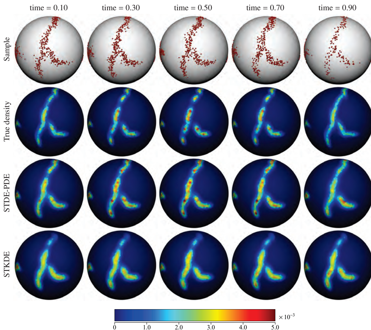
Figure 9: Simulation 3. Front view of the sample (first row), true density (second row), and mean estimates of STDE-PDE (third row), STKDE (fourth row), over 30 simulation repetitions, at different time instances. All the plots have the same color scale, with bluish colors corresponding to low density values.
