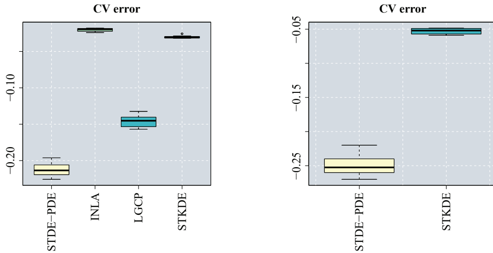
Figure 12: Left: Application to gastrointestinal infections; boxplots of 10-fold cross-validation errors for STDE-PDE and the competing methods introduced in Section 6.1, namely INLA, LGCP, and STKDE. Right: Application to earthquakes of large magnitude; boxplots of 10-fold cross-validation errors for STDE-PDE and STKDE.
