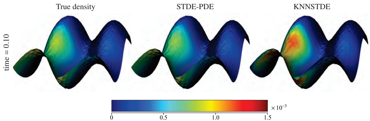
Figure H.2: Simulation 6: point pattern on a non-spherical two-dimensional manifold. True density (left), and mean estimates over 30 simulation repetitions obtained by the proposed STDE-PDE (center) and KNNSTDE (right), at a time instant at the beginning of the temporal domain [0, 1] . All the plots have the same color scale, with bluish colors corresponding to low density values.
