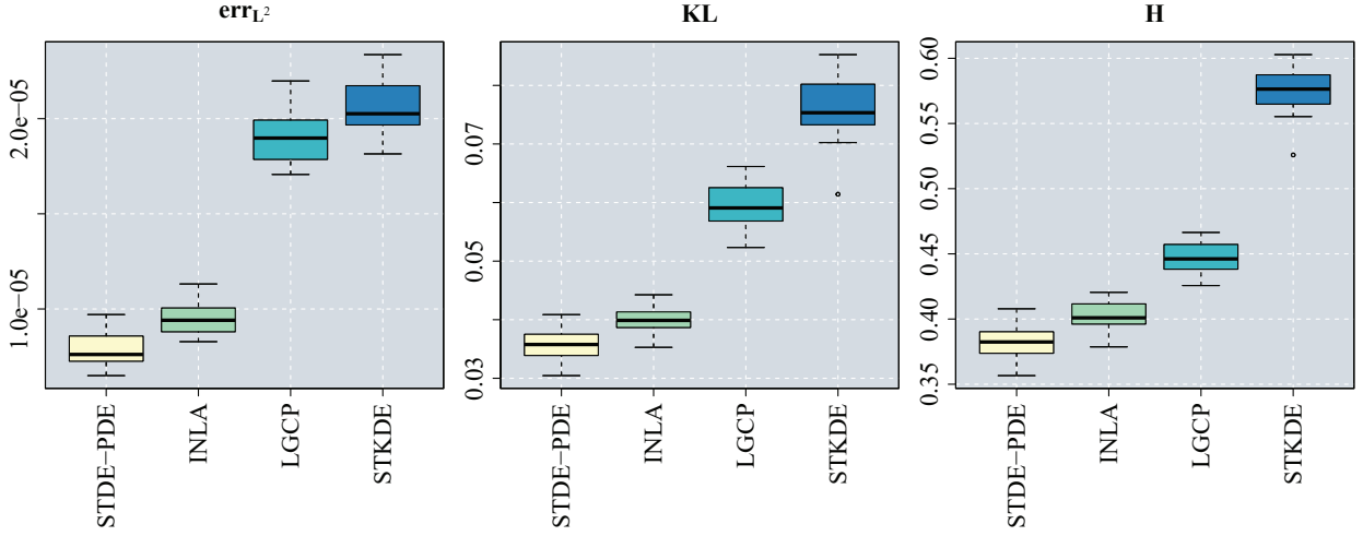
Figure G.1: Simulation 5, additional simulation on planar domain. Boxplots of L^2 -norm of the error (left), Kullback-Leibler divergence (center), and Hellinger distance (right) of the estimates provided by proposed STDE-PDE and the competing methods introduced in Section 6.1, namely INLA, LGCP, and STKDE, over 30 simulation repetitions.
