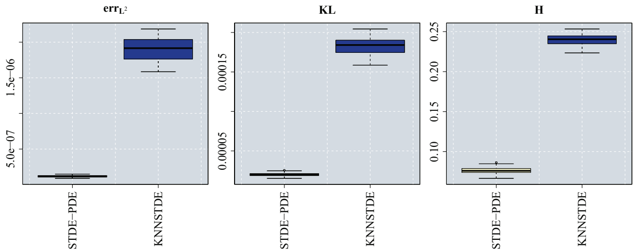
Figure H.3: Simulation 6: point pattern on a non-spherical two-dimensional manifold. Boxplots of L^2 -norm of the error (left), Kullback-Leibler divergence (center) and Hellinger distance (right), of the estimates provided by the proposed STDE-PDE, and the considered competing method KNNSTDE, over 30 simulation repetitions.
