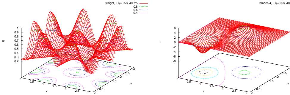
Figure 1: Weight w_C and solution u , for C_1 = \frac{97}{128} and C_2 = \frac{145}{256} .
