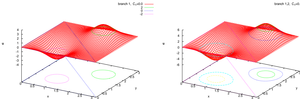
Figure 2: Starting point and bifurcation point on branch 1.
