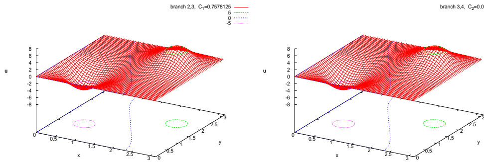
Figure 3: Two points on branch 3.
