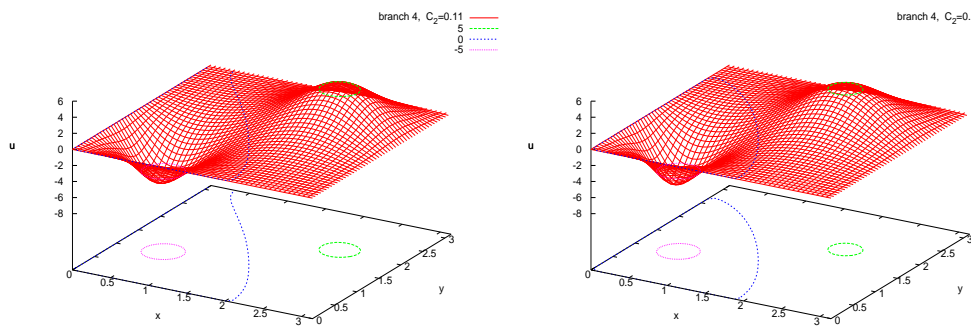
Figure 4: Two points on branch 4.
