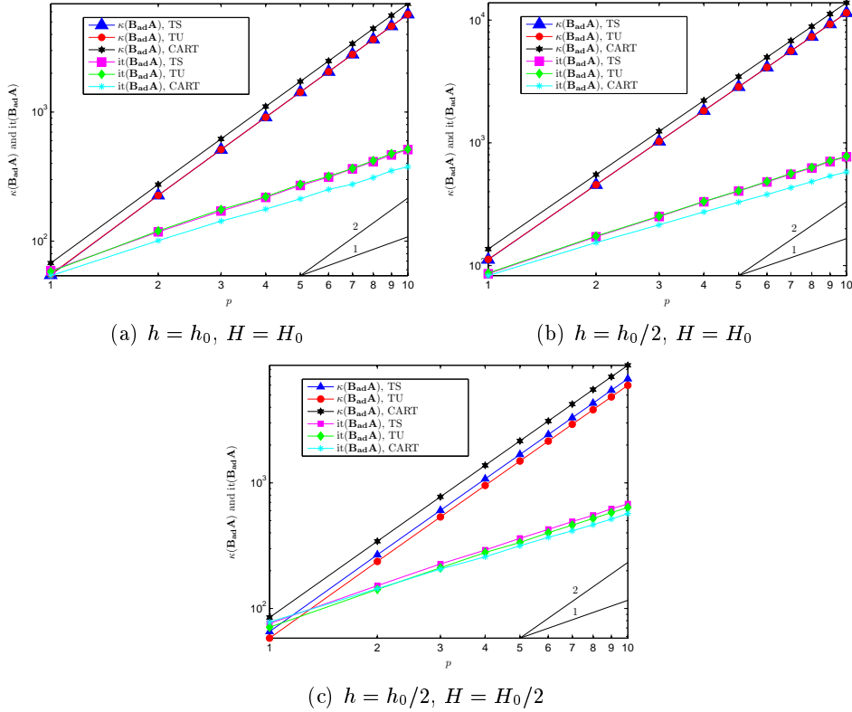
Figure 5: Condition number estimates of the preconditioned system and corresponding iteration counts versus the polynomial degree p on structured triangular grids (TS), unstructured triangular grids (TU) and Cartesian grids (CART) for different discretization steps.
