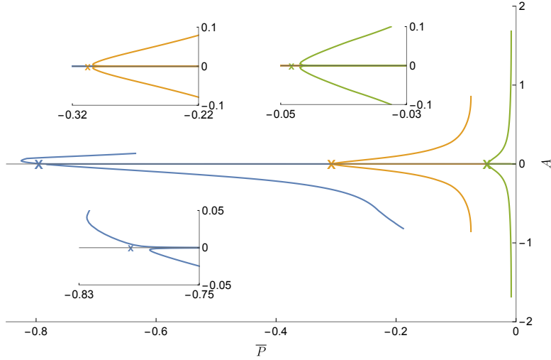
Figure 9: Post-buckling behavior showing \bar{P} versus the dimensionless amplitude of the deformation at the free surface, setting \bar{V} = 0.3 , \mu^e/\mu^d = 10 , t^d = 0.9 , and t^e = 0.9, 0.95, 1 (blue, orange, and green lines, respectively). The \times marker denotes the theoretical buckling threshold.
