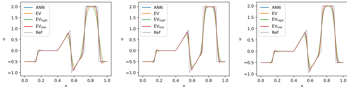
Figure 10: Test case 3: solution at T = 0.4 for k = 1, 3, 5 (from left to right).
