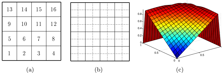
Figure 1: (a) Subdomain ordering for N = 16 ; (b) initial coarse (solid line) and fine (dashed line) meshes; (c) the exact solution (4) for \varepsilon = 10^{-2} (right).
