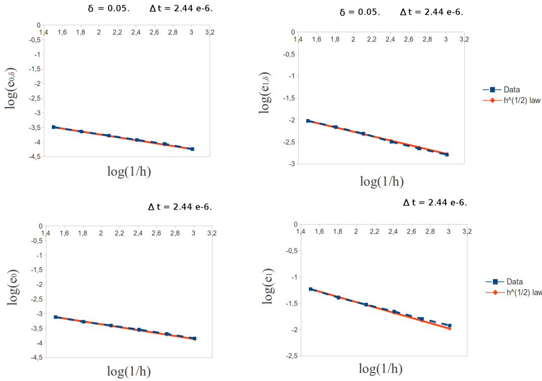
Figure 1: Test case 1. Values of \log(e_{0,\delta}) , \log(e_{1,\delta}) , \log(e_0) , \log(e_1) vs \log(1/h) , for \delta = 0.05 , \Delta t = 2.44 \cdot 10^{-6} , and an exact decay law proportional to h^{1/2} , where e_{0,\delta} := \|c - C_h^+\|_{L^\infty(0,T;L^2(D_\delta^+(t)))} , e_{1,\delta} := \left\| \frac{\partial}{\partial x}(c - C_h^+) \right\|_{L^\infty(0,T;L^2(D_\delta^+(t)))} , e_0 := \|c - C_h^+\|_{L^\infty(0,T;L^2(\Omega))} , e_1 := \left\| \frac{\partial}{\partial x}(c - C_h^+) \right\|_{L^\infty(0,T;L^2(\Omega))} .
