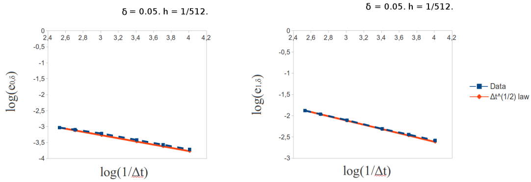
Figure 2: Test case 1. Values of \log(e_{0,\delta}) , \log(e_{1,\delta}) , vs \log(1/\Delta t) , for \delta = 0.05 , h = 1/512 , and an exact decay law proportional to \Delta t^{1/2} , where e_{0,\delta} := \|c - C_h^+\|_{L^\infty(0,T;L^2(D_\delta^+(t)))} , e_{1,\delta} := \left\| \frac{\partial}{\partial x}(c - C_h^+) \right\|_{L^\infty(0,T;L^2(D_\delta^+(t)))} .
