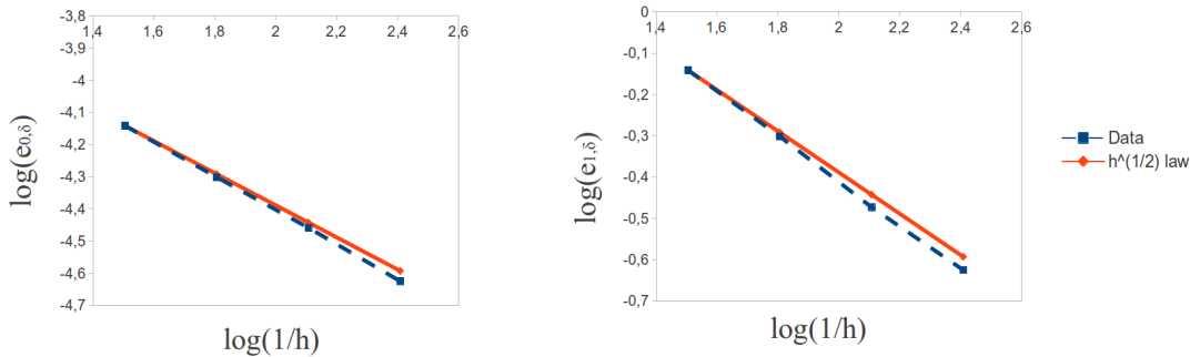
Figure 5: Test case 3. Values of \log(e_{0,\delta}) and \log(e_{1,\delta}) vs \log(1/h) , for \delta = 0.05 , for \Delta t = 2.44 \cdot 10^{-6} , and an exact decay law proportional to h^{1/2} , where e_{0,\delta} := \|c - C_h^+\|_{L^\infty(0,T;L^2(D_\delta^+(t)))} , e_{1,\delta} := \left\| \frac{\partial}{\partial x}(c - C_h^+) \right\|_{L^\infty(0,T;L^2(D_\delta^+(t)))} .
