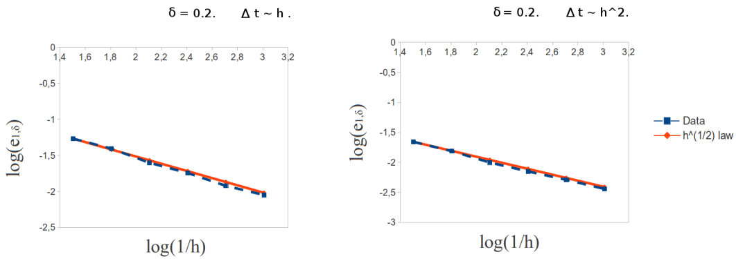
Figure 3: Test case 1. Values of \log(e_{1,\delta}) , vs \log(1/h) , for \delta = 0.2 , with \Delta t \sim h and \Delta t = h^2 , and an exact decay law proportional to h^{1/2} , where e_{1,\delta} := \left\| \frac{\partial}{\partial x}(c - C_h^+) \right\|_{L^\infty(0,T;L^2(D_\delta^+(t)))} .
