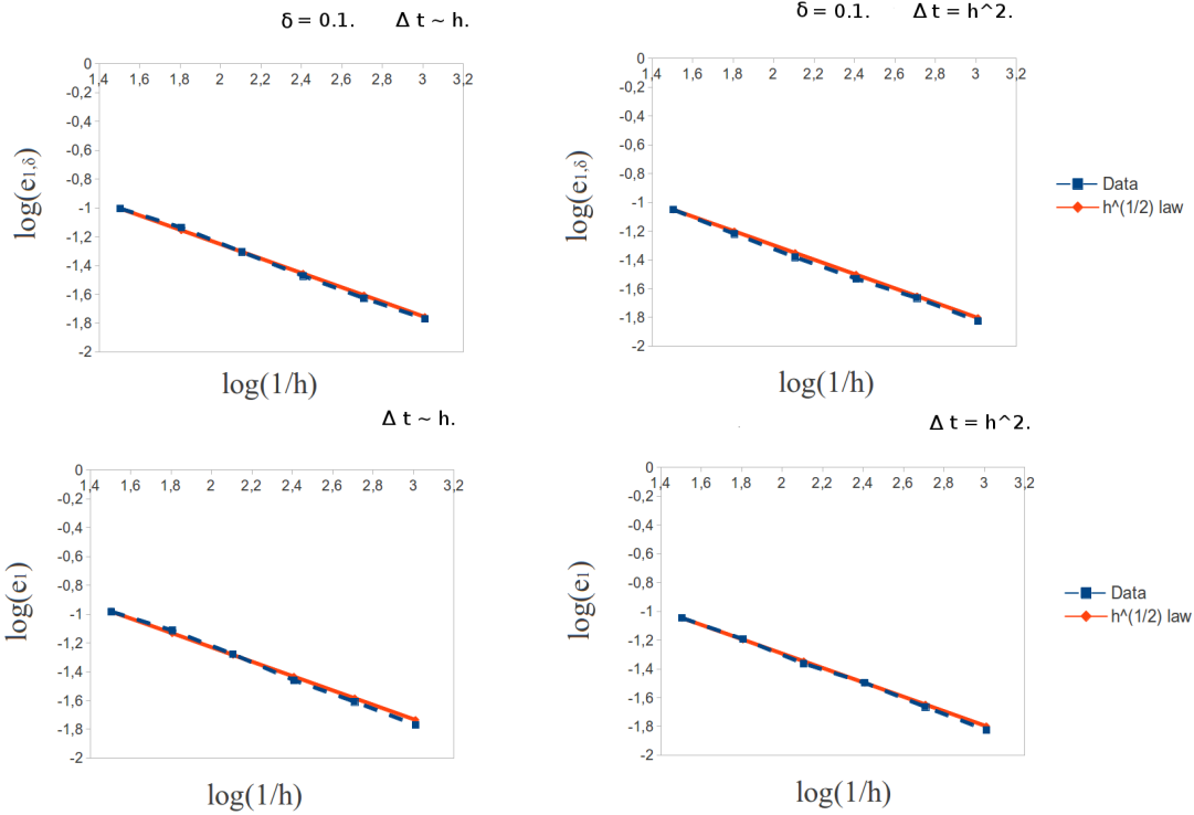
Figure 4: Test case 2. Values of \log(e_{1,\delta}) and \log(e_1) vs \log(1/h) , for \delta = 0.1 , for the cases \Delta t \sim h and \Delta t = h^2 , and an exact decay law proportional to h^{1/2} , where e_{1,\delta} := \left\| \frac{\partial}{\partial x}(c - C_h^+) \right\|_{L^\infty(0,T;L^2(D_\delta^+(t)))} ,
