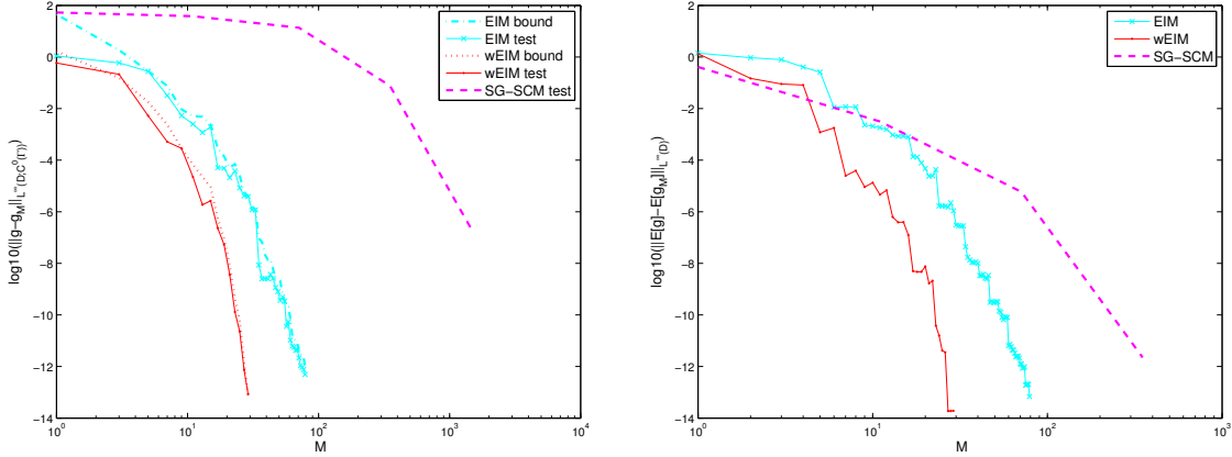
Figure 4.2: Comparison of convergence property of EIM, wEIM and SG-SCM in different norms. Left: decreasing of the error \|g - g_M\|_{L^\infty(D; C^0(\Gamma))} ; Right decreasing of the error \|\mathbb{E}[g] - \mathbb{E}[g_M]\|_{L^\infty(D)} ; K=5
