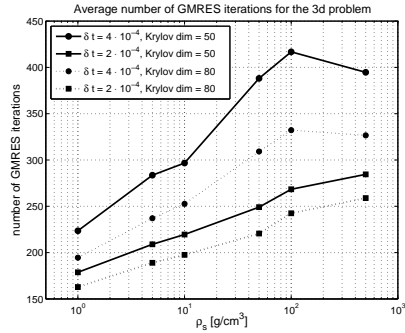
(b) Dependence with \delta t
