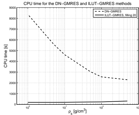
Figure 10: CPU time for the ILUT-GMRES and the DN-GMRES methods as the structure density varies.
