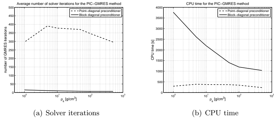
Figure 9: (a) Average number of GMRES iterations and (b) CPU time for the PIC-GMRES method with different preconditioners as the structure density varies.
