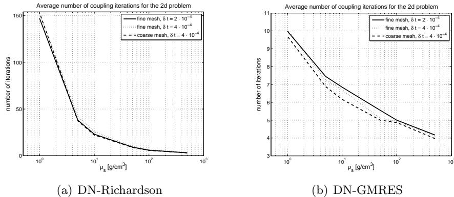
Figure 2: Average number of coupling iterations for (a) the DN-Richardson and (b) DN-GMRES methods as the structure density varies. Comparison for different meshes and different time step values.
