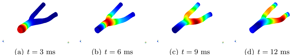
Figure 7: Propagation of the initial pressure pulse, moving from the inflow to the outflow section. Solution at every 3 ms.
