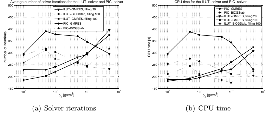
Figure 8: (a) Average number of solver iterations and (b) CPU time for the ILUT-solver and the PIC methods as the structure density varies.
