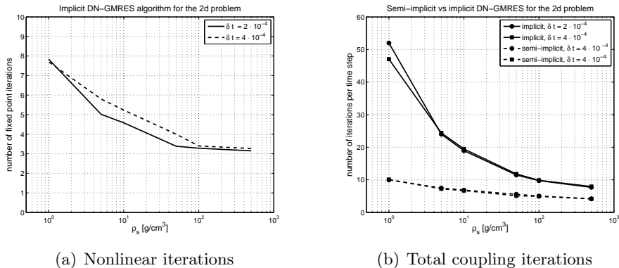
Figure 3: (a) Average number of fixed point iterations for the implicit version and (b) average number of total GMRES iterations per time step for the implicit and semi-implicit versions, for different structure densities and time steps values.
