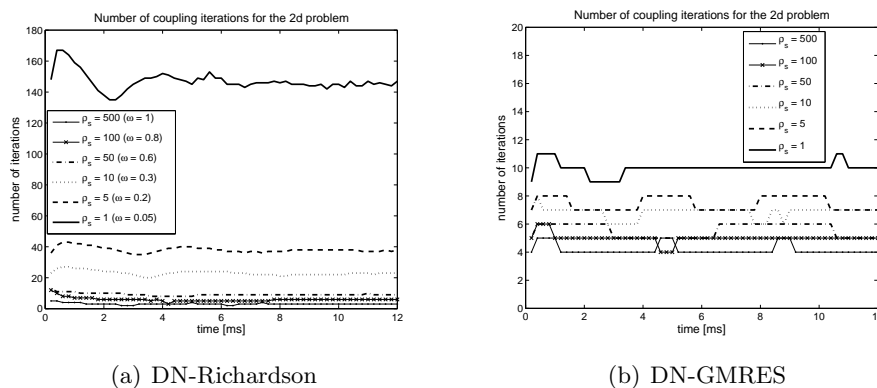
Figure 1: Number of coupling iterations needed to satisfy the convergence criterion at each time step for (a) the DN-Richardson and (b) DN-GMRES methods.
