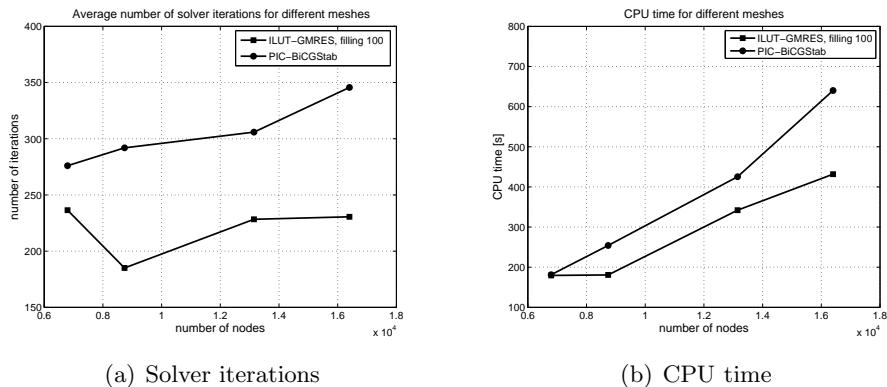
Figure 11: (a) Average number of solver iterations and (b) CPU time for the ILUT-GMRES and the PIC-BiCGStab methods for different meshes.
