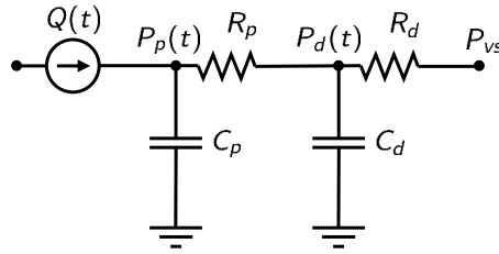
FIGURE 1 Visual representation of the two-stage Windkessel model of Eq. (1). In this electrical analogy, current represents blood flux, while voltage represents blood pressure. The heart is represented as a current generator, while the arterial network comprises dissipative and compliant elements, represented by resistances and capacitors, respectively.
