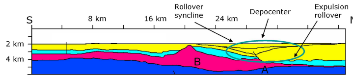
(a) Cretaceous phase 2
