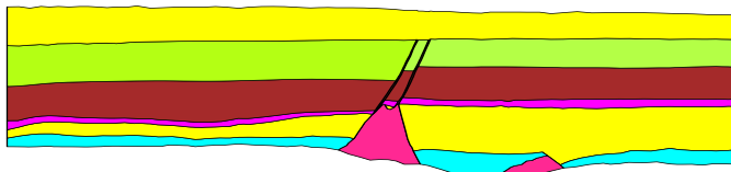
(e) Present Day
