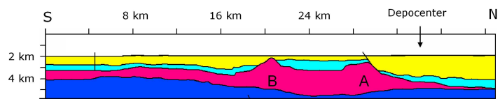
(c) Cretaceous phase 1
