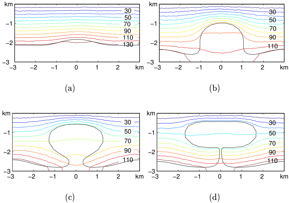
Figure 5. Thermal anomaly induced by a growing salt diapir in sedimentary basin. The figure represents the the isolines for temperature ( ^{\circ}C ).
