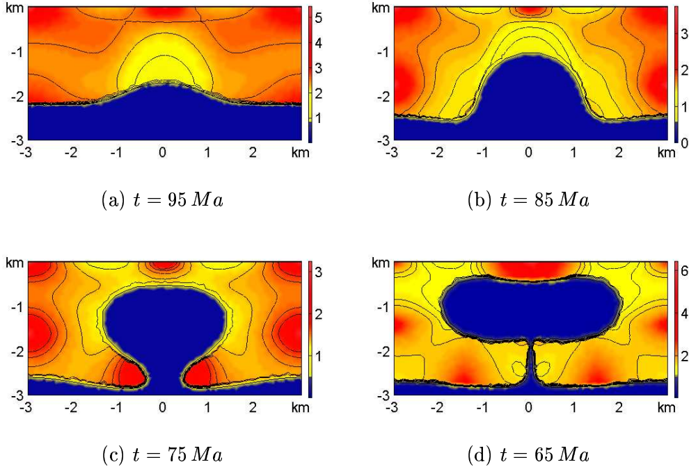
Figure 2. Evolution of a single salt diapir in a non-Newtonian overburden modeled with power-law rheology. The power law exponent is r = 1.7 . In these pictures the evolution of the apparent viscosity ( Pa\ s ) (together with its isolines) of the overburden is shown.
