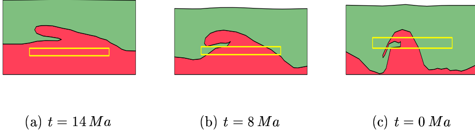
Figure 4. Evolution of a salt tongue in an extensional basin. The boxes represent the salt flux area. The evacuation intervals are [18 Ma, 14 Ma] , [9 Ma, 8 Ma] , [4 Ma, 0 Ma] .
