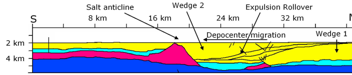
(b) Cretaceous phase 3
