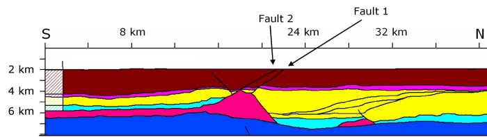
(b) early Tortonian
