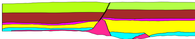
(c) Early Tortonian (11 Ma)
