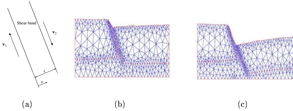
Figure 3. Development of a fault and computational mesh evolution.
