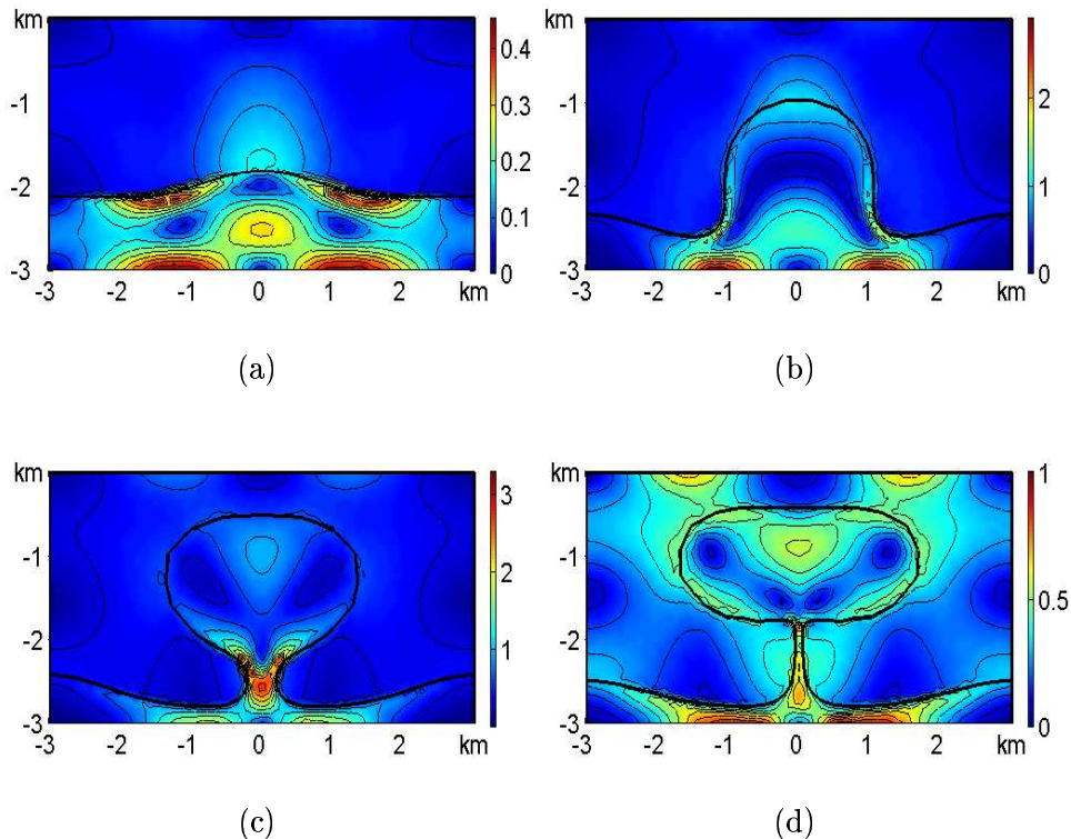
Figure 6. Creeping deformation of a salt diapir. Evolution of the strain rate 10^{-13}(s^{-1}) .
