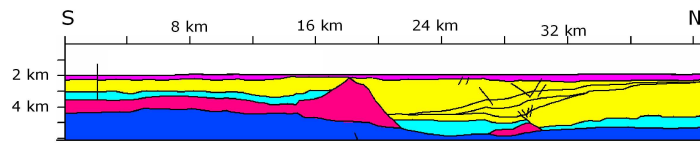
(a) late Oligocene
