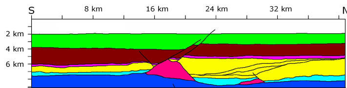
(c) Messinian
