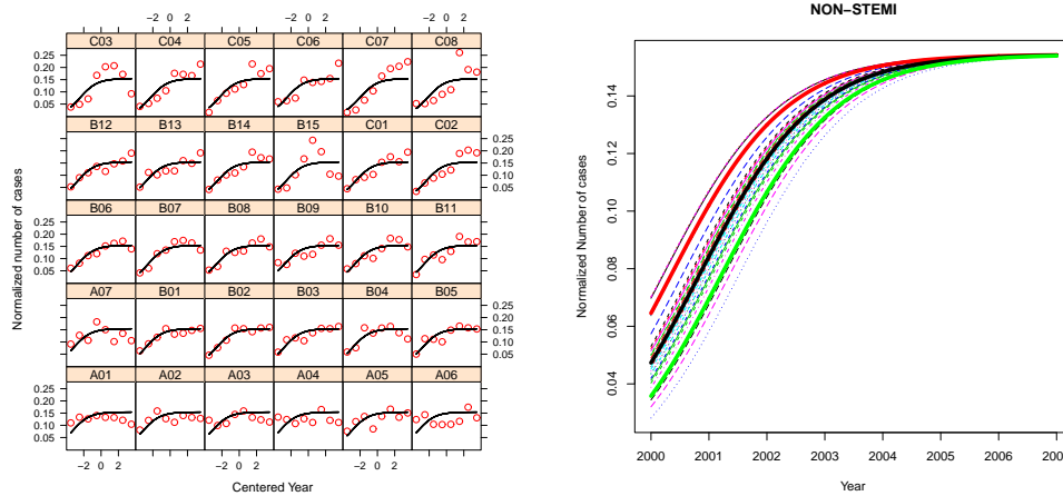
Figure 4: Estimated logistic growth curves for different medical institutions.
