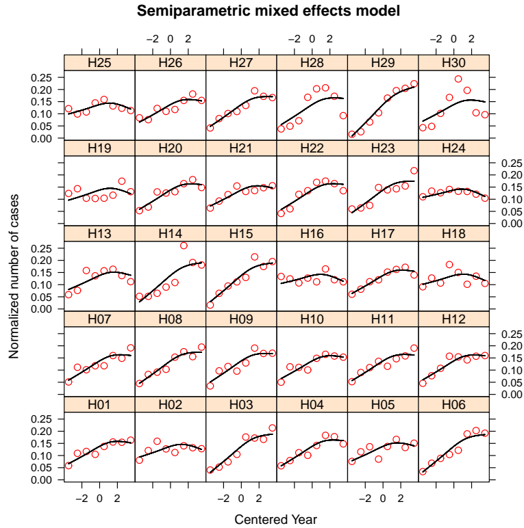
Figure 2: Estimated growth curves through model 1 together with the original data.
