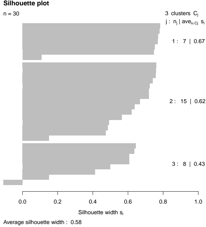
Figure 3: Silhouette plot of PAM procedure on the estimated inflection points with k = 3 clusters.
